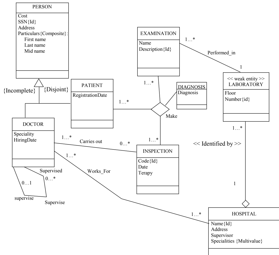
Figura 1: UML class diagram of a system managing hospital information
